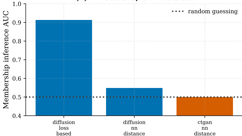
(b) All attacks, ULB dataset
