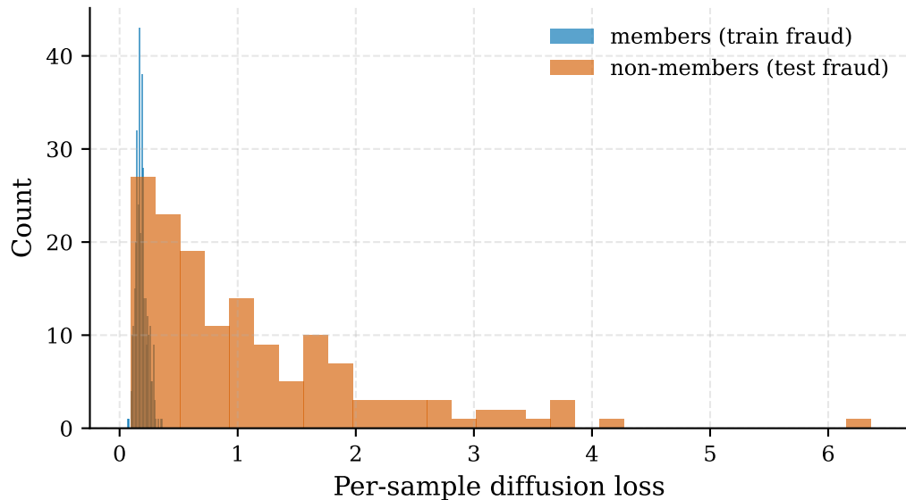
(a) Loss-based attack (diffusion-specific) AUC=0.913
